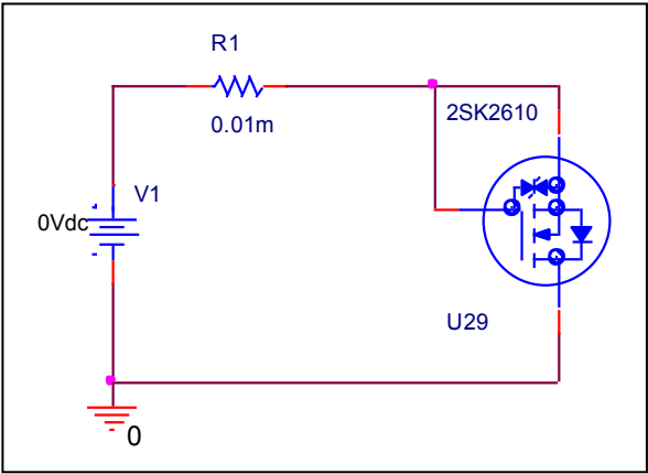
Evaluation Circuit
