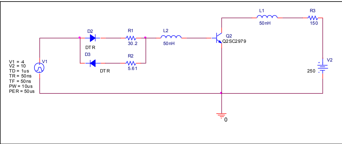
Evaluation circuit
