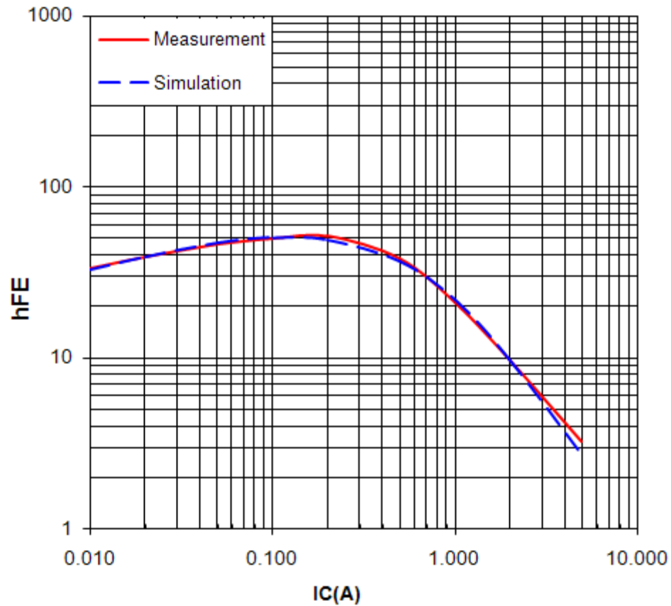
Simulation Result
