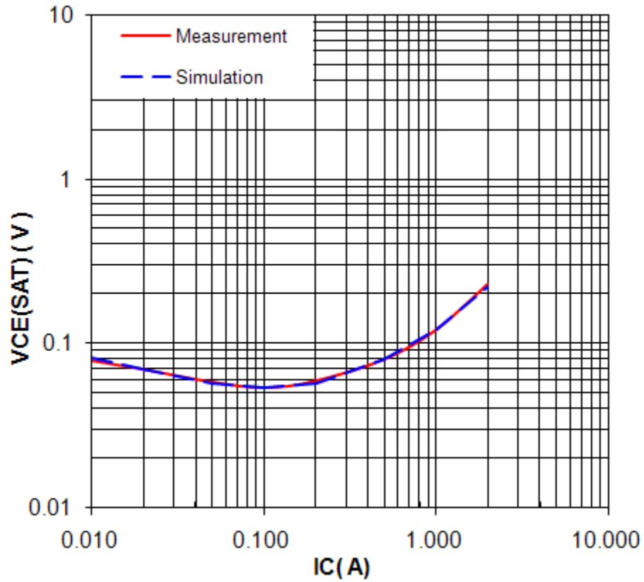
Simulation Result
