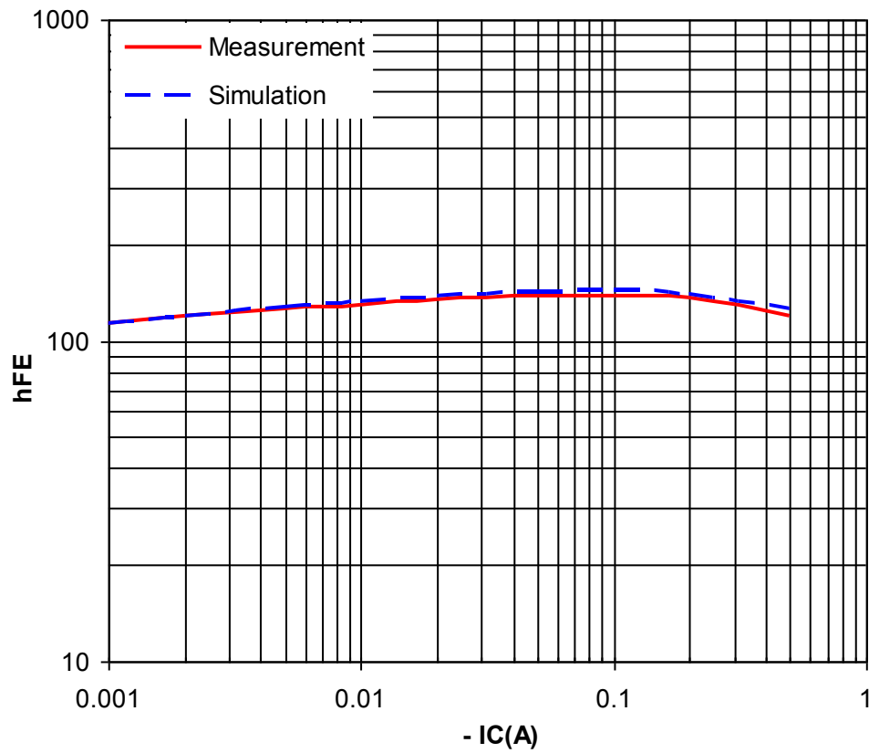
Circuit Simulation Result
