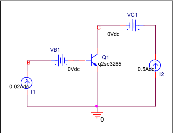
Simulation result
